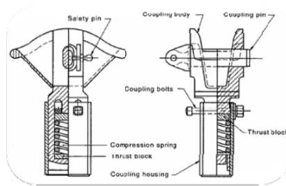
Spring Cushioned Female Coupling
